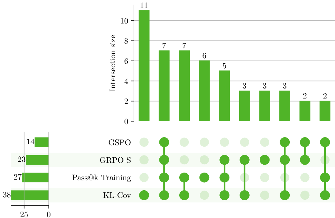
Expansion Intersections (pass@256 Base=0, RL=1), Model: EuroLLM-9B-Instruct
